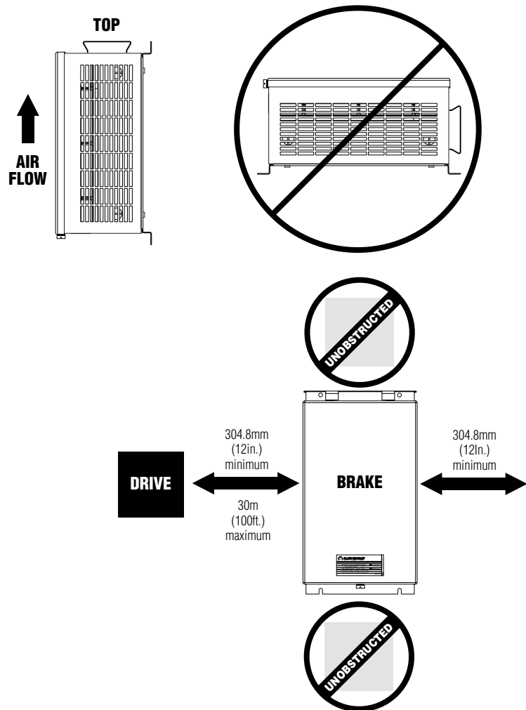
Recommended Brake Mounting Configuration
