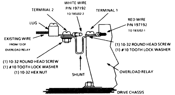
15 & 20 HP 1334 DRIVES WITH OVERLOAD RELAY
