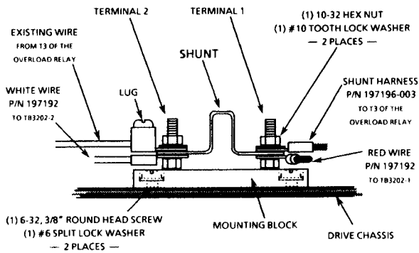
25 HP 1334 DRIVES WITH OVERLOAD RELAY
