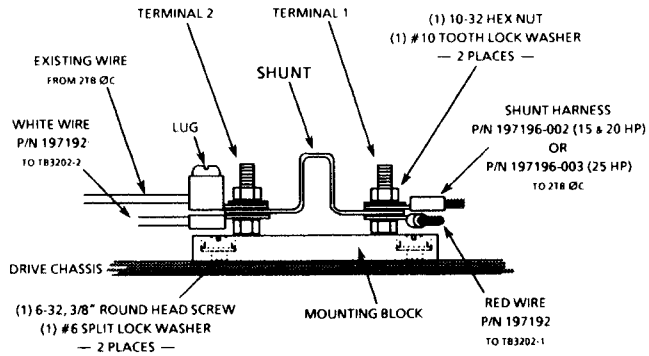
ALL 1334 DRIVES WITHOUT OVERLOAD RELAY
