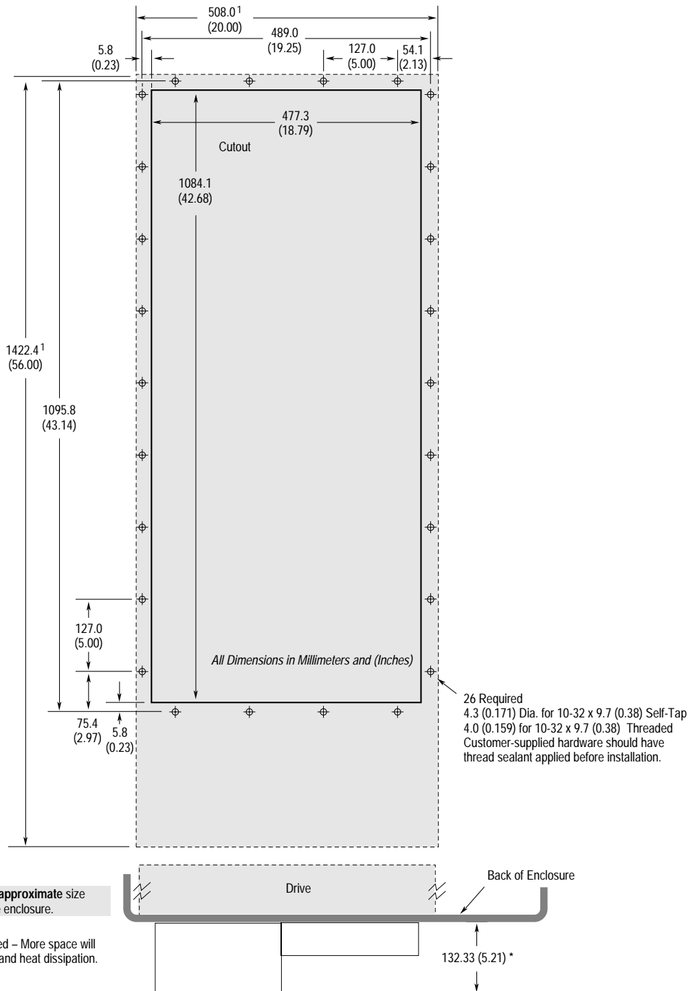
Figure 1.6 Heat Sink Through-the-Back Mounting – Frame E
