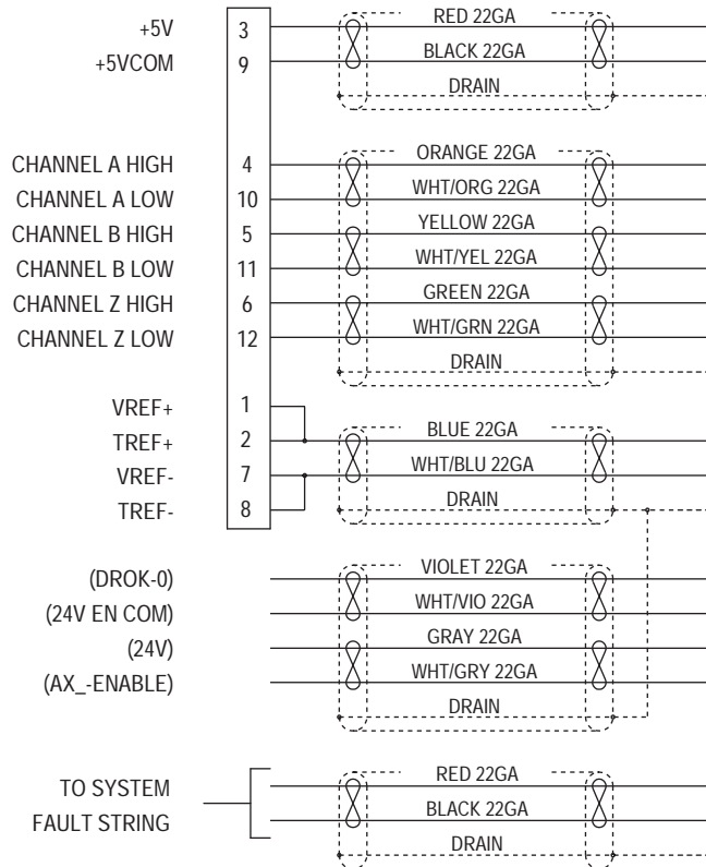
Figure 2 1394-CFLAE01, -03, -08, and -15 Connector Cable Pinouts
