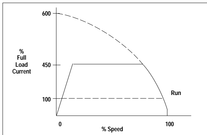
Figure 5 Current Limit Acceleration
