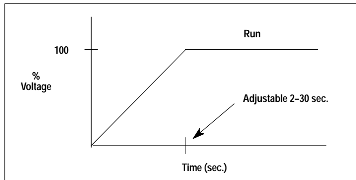
Figure 4 Soft Start
