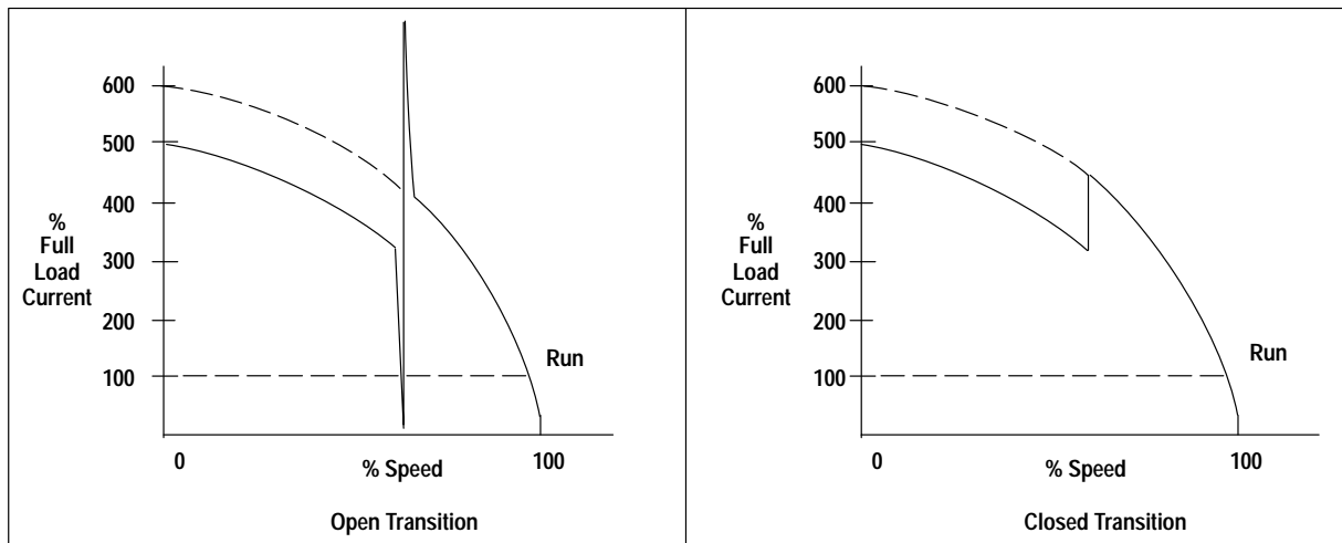
Figure 2 Open Circuit Transition vs. Closed Circuit Transition
