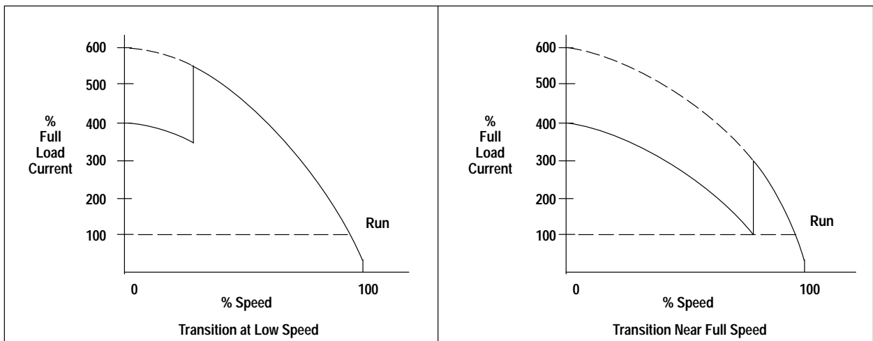
Figure 3 Transition at Low Speed vs. Transition Near Full Speed
