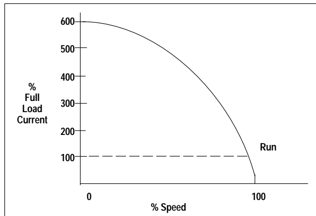
Figure 1 Full Load Current vs. Speed
