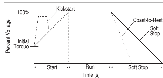
SMC-3 Controller (Softer Starter)
