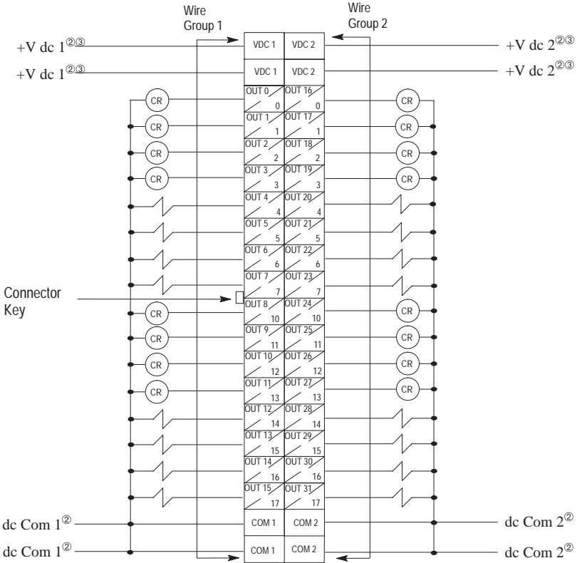
1746-OB32 5–50V dc Transistor Output Sourcing
