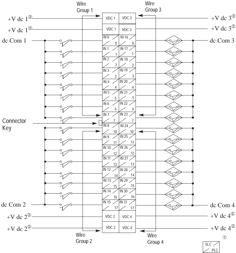
1746-IV32 24V dc Sourcing
