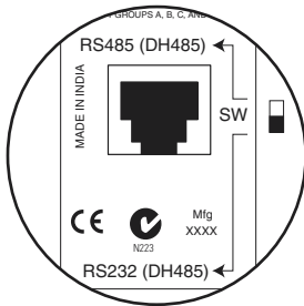
Set for RS-232 port
