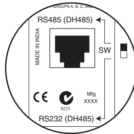
Set for RS-485 port
