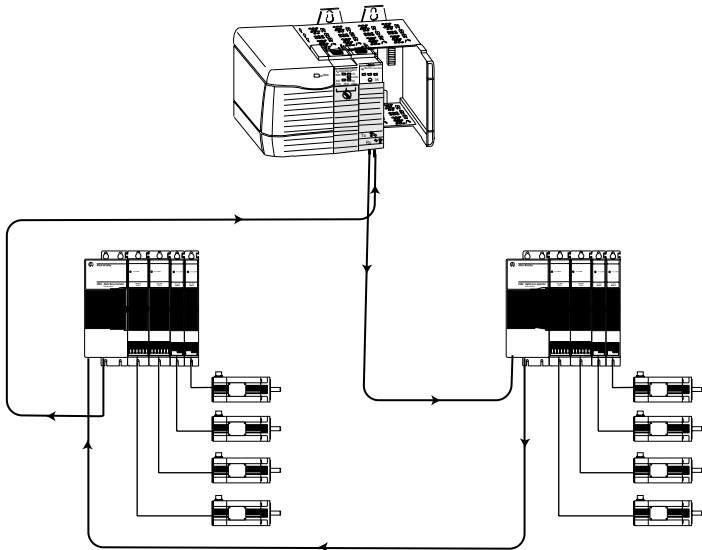
Figure 6 Ring topology with 1394C-SJTxx-D
