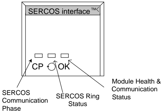
Figure 7 LED Location and Description
