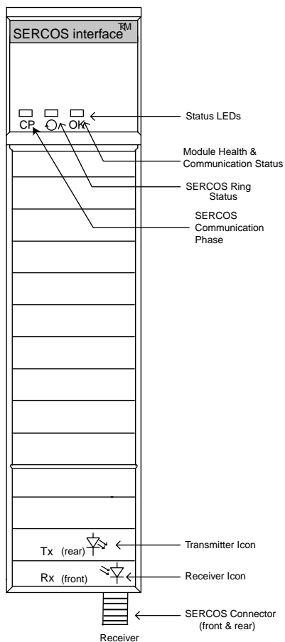
Figure 1 Front View of the Module
