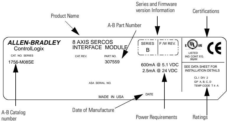
Figure 3 1756-MxxSE Product Label
