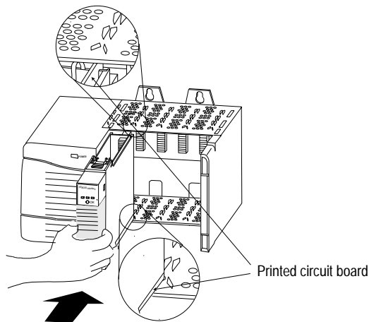
Figure 4 Align Module
