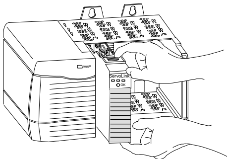
Figure 9 Pull Module Out
