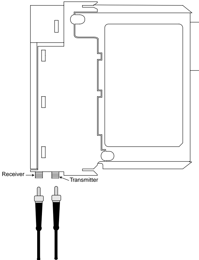
Figure 2 Side View of the Module Showing Fiber Optic Cable Connections
