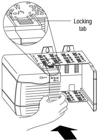
Figure 5 Seat the Module
