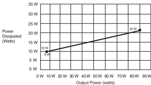
1768-PB3 Power Dissipation
