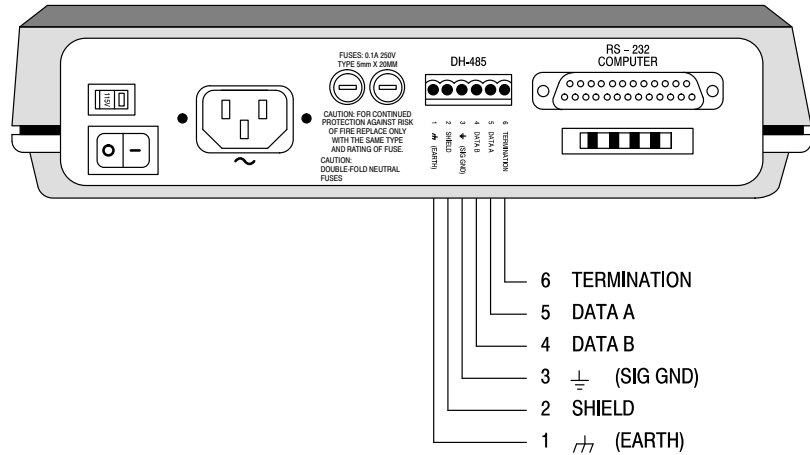
Figure 1 KF3 Pinouts
