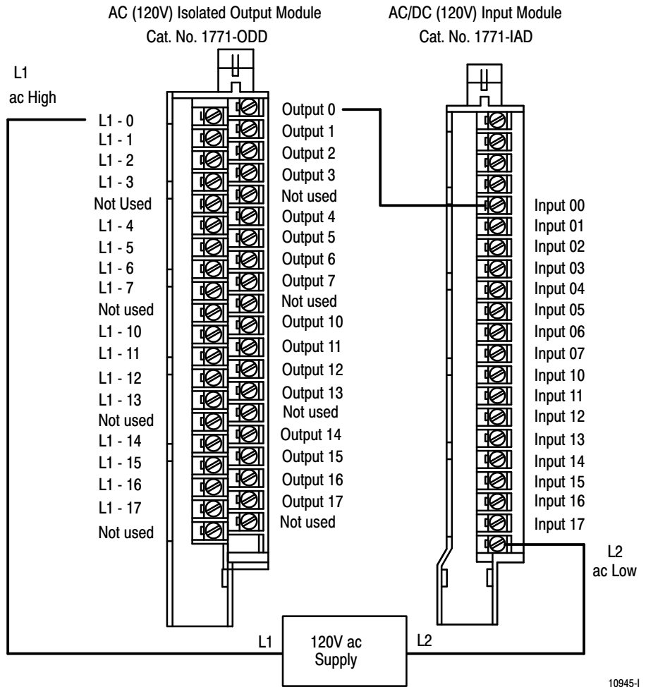
Figure 2 Driving an Input with an Output
