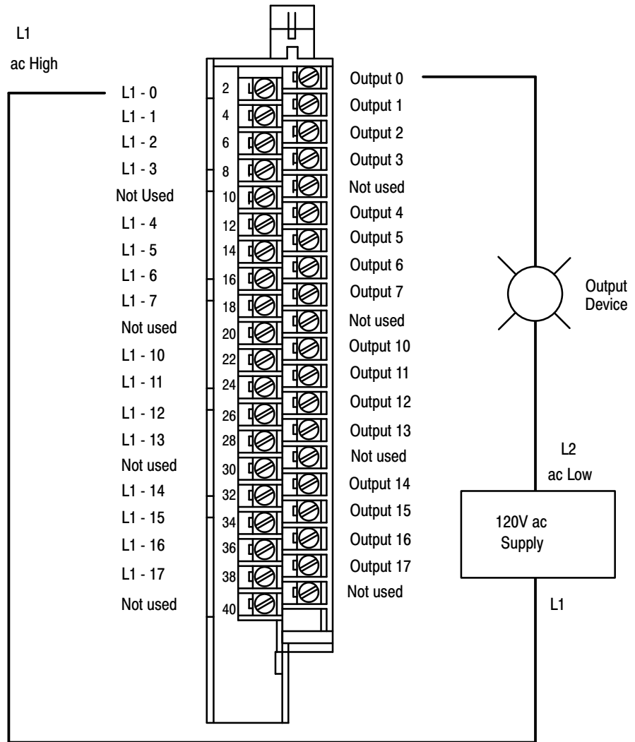
Figure 1 Connection Diagram for the 1771-ODD Isolated Output Module
