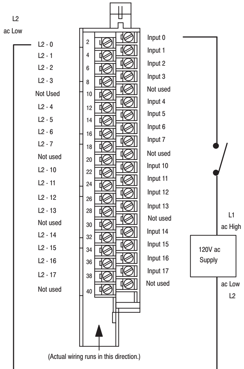
Figure 1 Connection Diagram for the 1771-ID16GM ac (120V) Isolated Input Module
