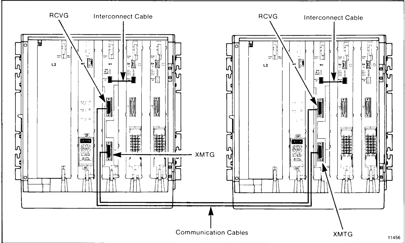
Figure 1 Typical Installation of Memory Communication Cable Assembly
