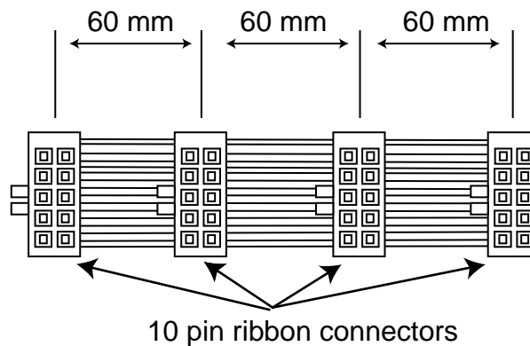
Figure 1 1784-PMCSY4 Cable
