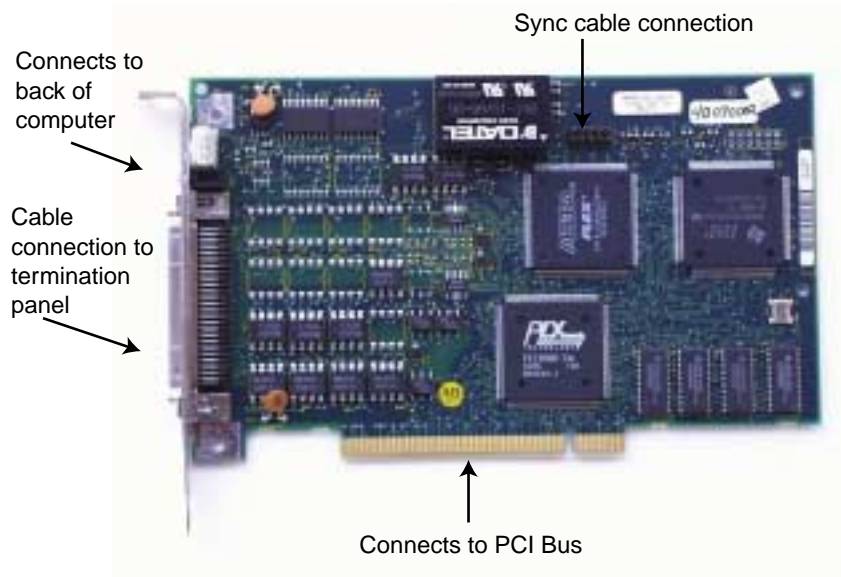
Figure 2 Side View of the 1784-PM02AE Card
