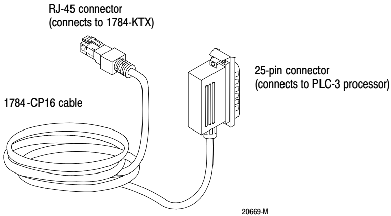
Figure 1 1784-CP16 cable
