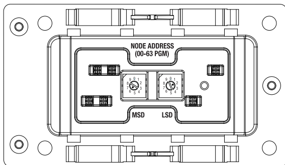
Bottom View of Module Example: Node address is set at 62, see small black dots.
