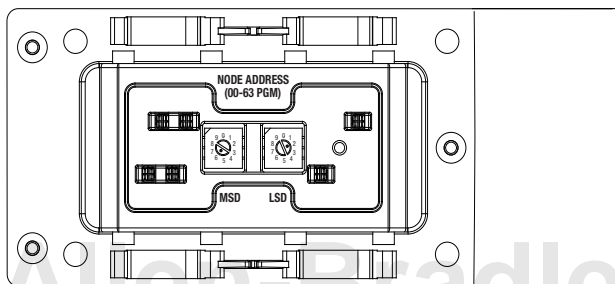
Bottom View of Module Example: Node Address is set at 62, see small black dots.
