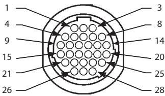
Front of Tyco AMP 205839-3 Housing
