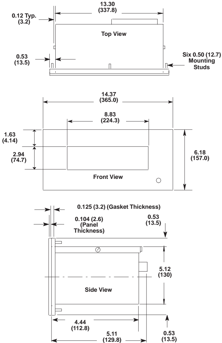
Figure 1 Four Line Dimensions
