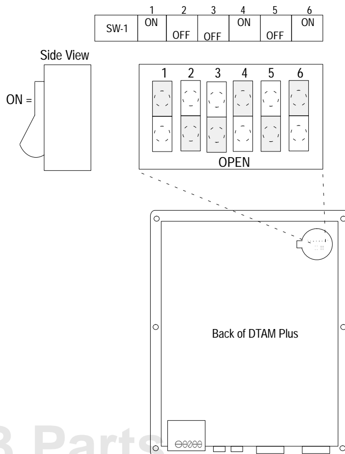
Figure 6.1 DIP Switch Settings for Download
