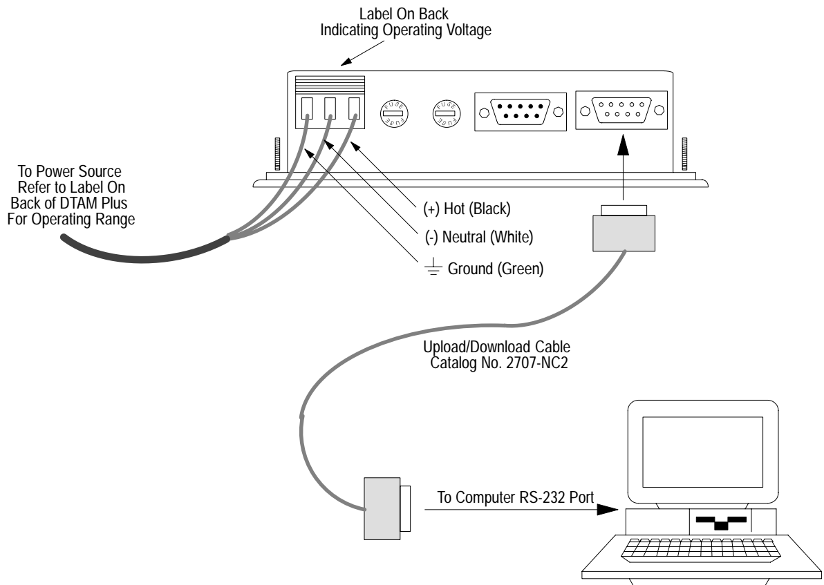
Figure 6.2 Power and Download Connections
