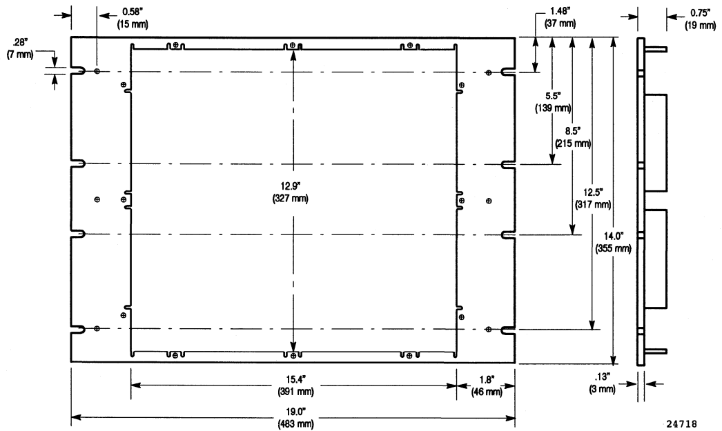
Figure 1 19-Inch Rack Mount Assembly for Touch Screen Terminals
