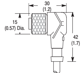
Right Angle Female
