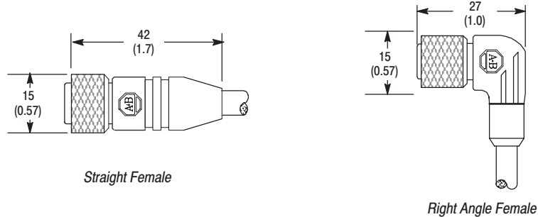
Right Angle Female
