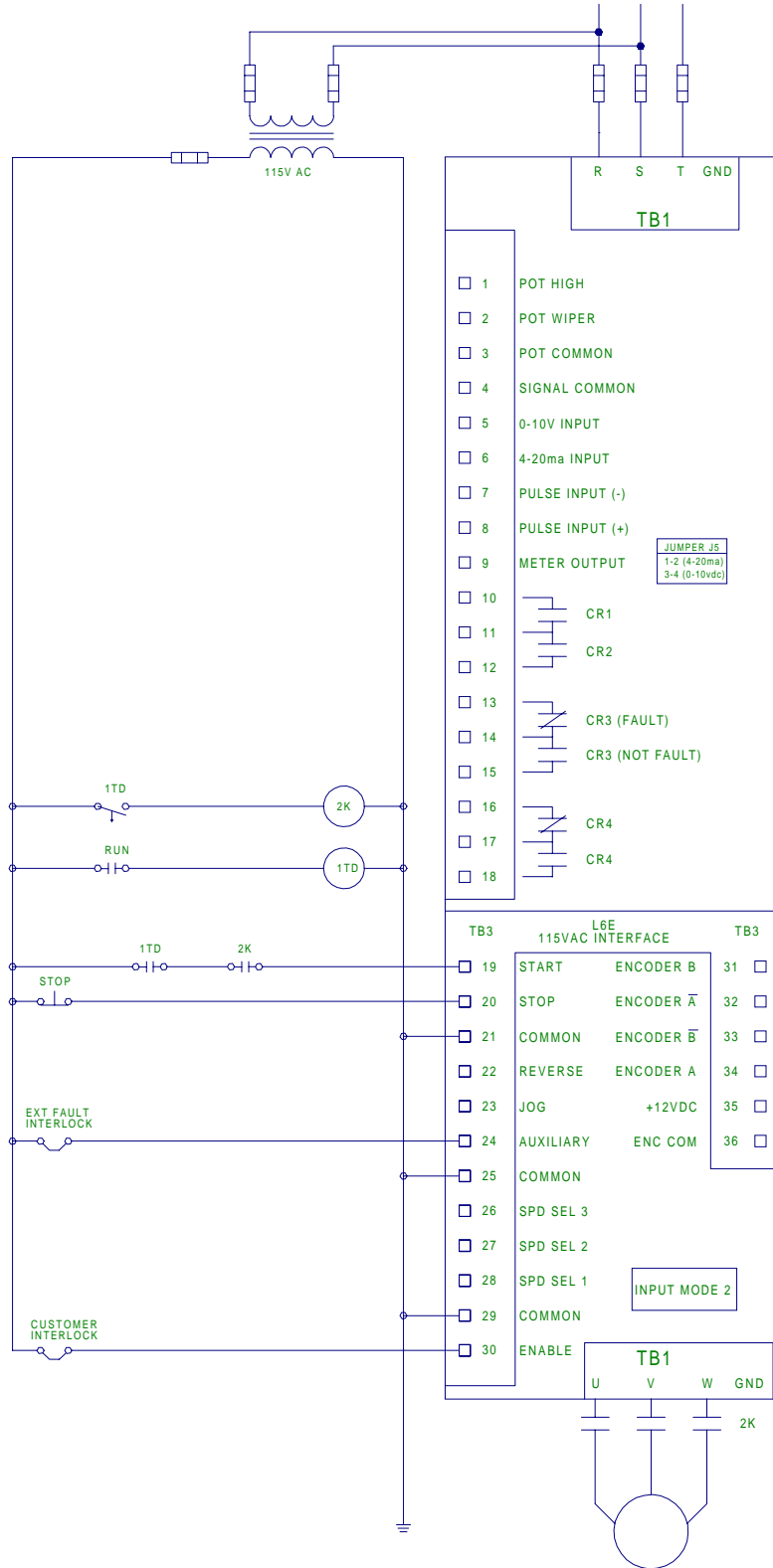
FIGURE 1 OUTPUT CONTACTOR WITH TIMER CONTROL
