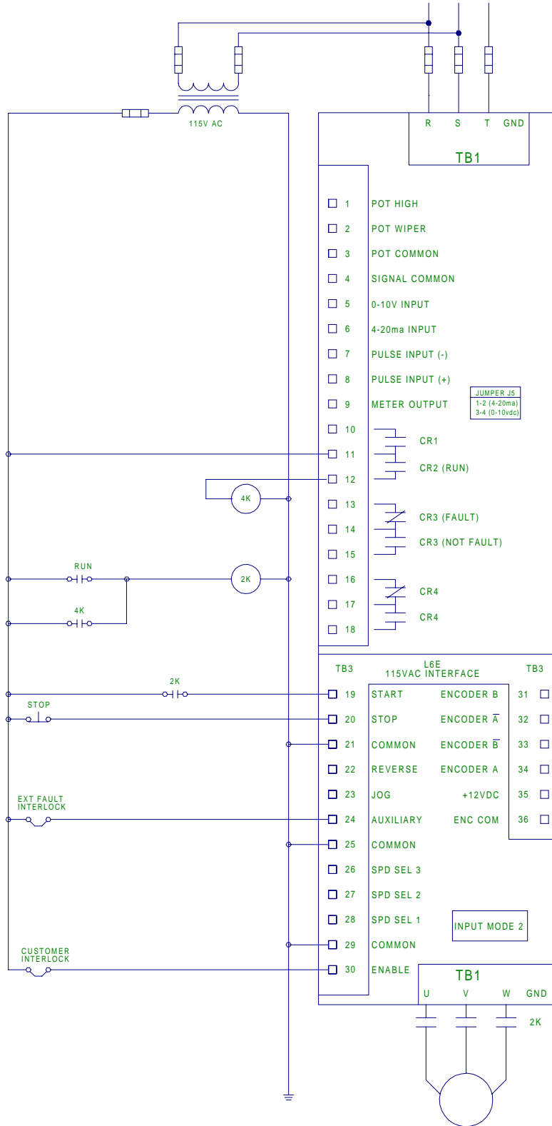
FIGURE 1 OUTPUT CONTACTOR WITH RUN CONTACT CONTROL
