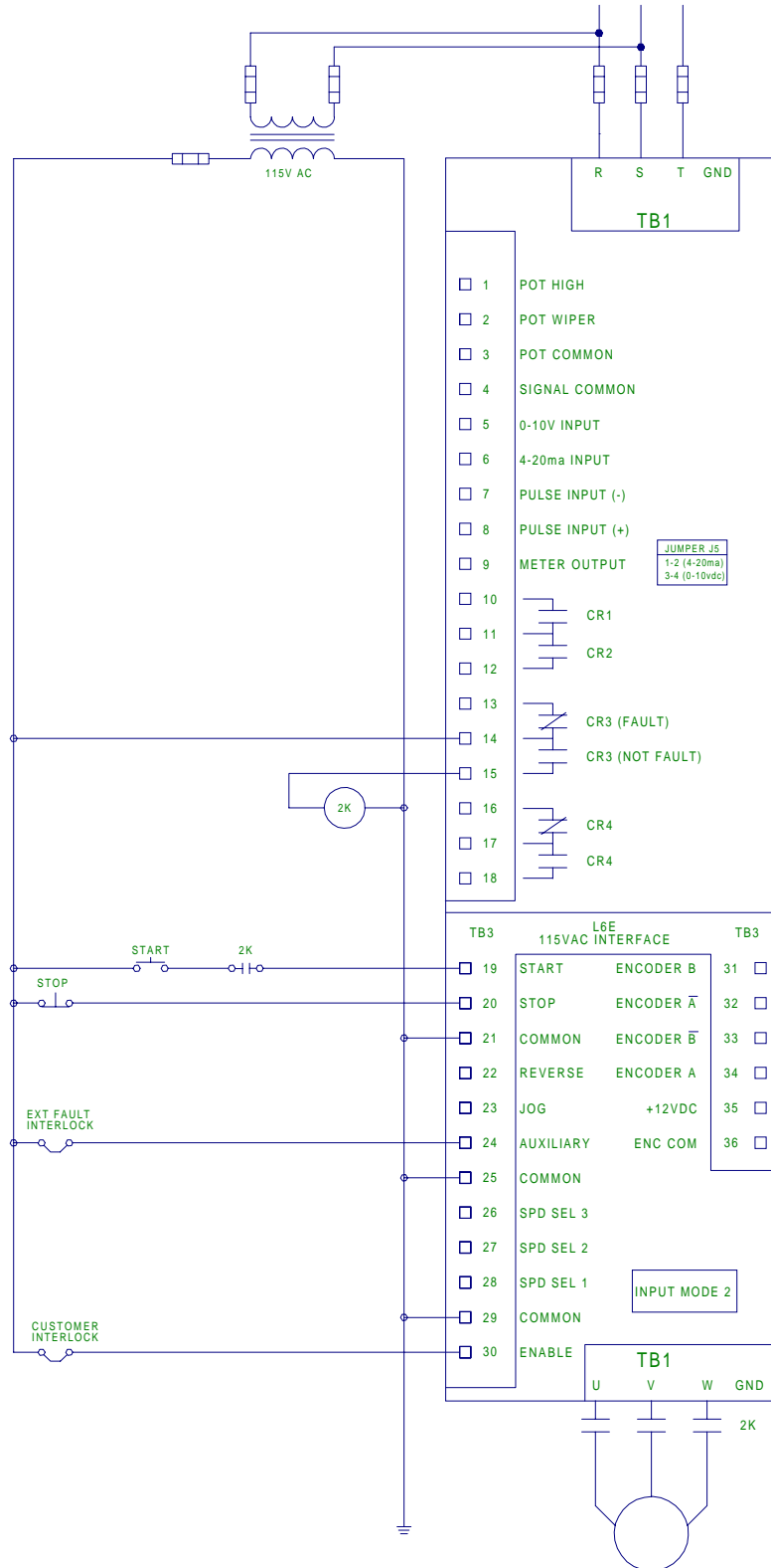
FIGURE 1 OUTPUT CONTACTOR WITH FAULT CONTACT CONTROL
